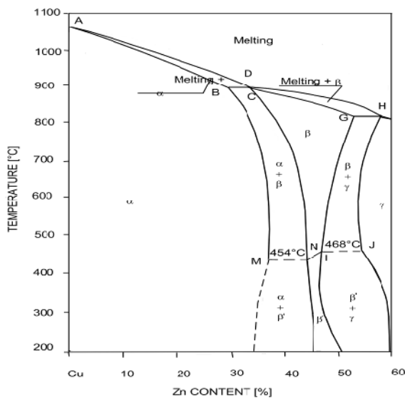
Fig. 5. Binary diagram copper-zinc
