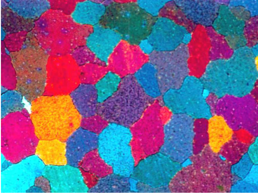
a) polyhedral grains of \beta' phase, polarized light, mag. 100 x
