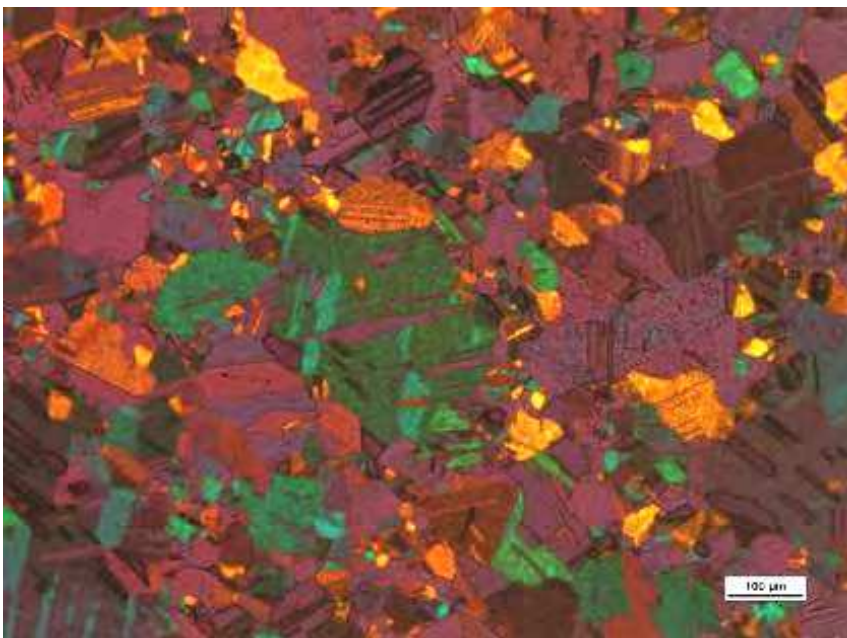
b) size and orientation of grains, polarized light, etched \text{K}_2\text{Cr}_2\text{O}_7
